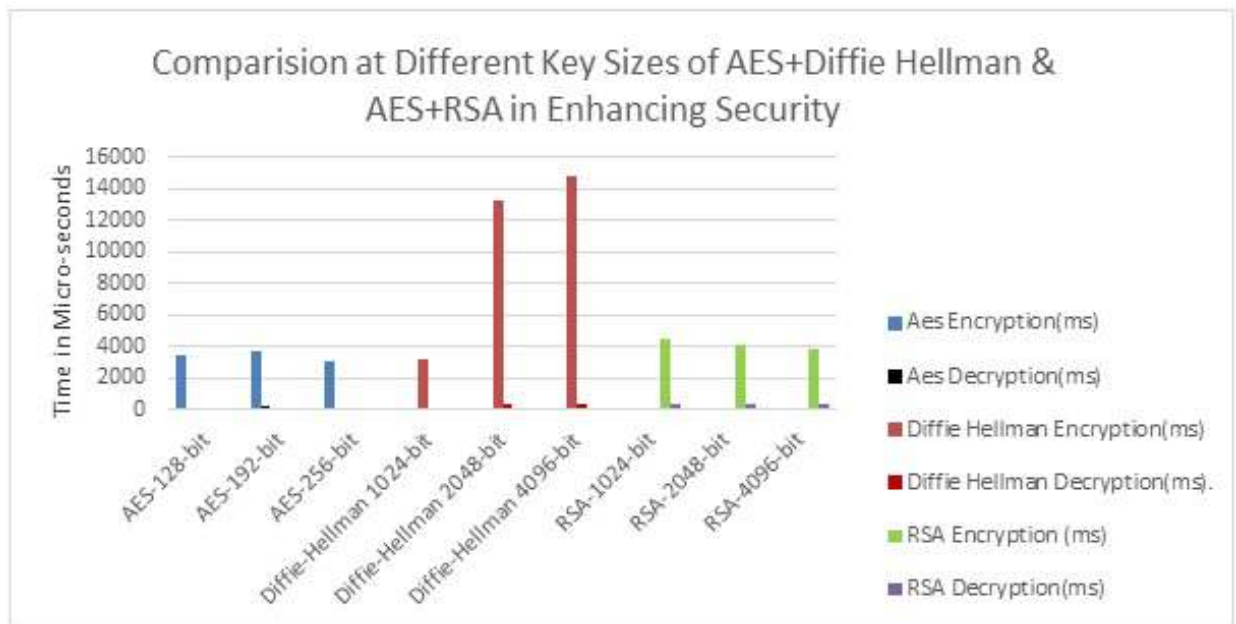
Figure 5. Comparisons based on different key sizes of AES, Diffie-Hellman & RSA
