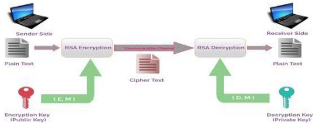
Figure 2. RSA Algorithm and its Diagrammatic Representation
