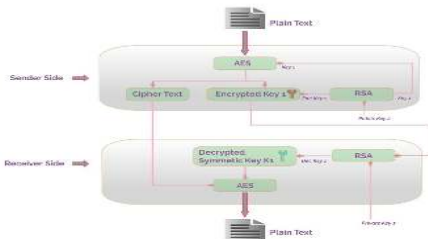
Figure 3. AES & RSA Encryption/Decryption Using the Hybrid/Mixed Algorithm Approach
