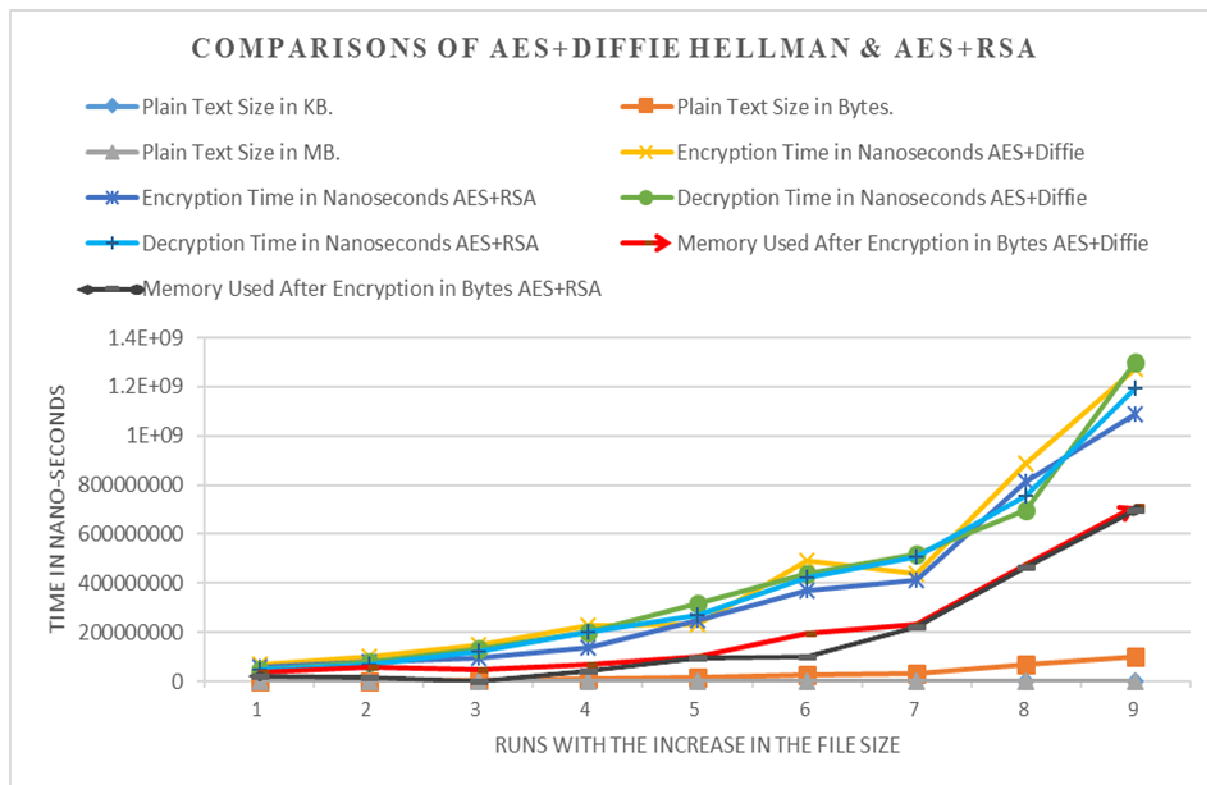
Figure 4. Performance of Proposed Algorithm (Time & Memory Usage)
