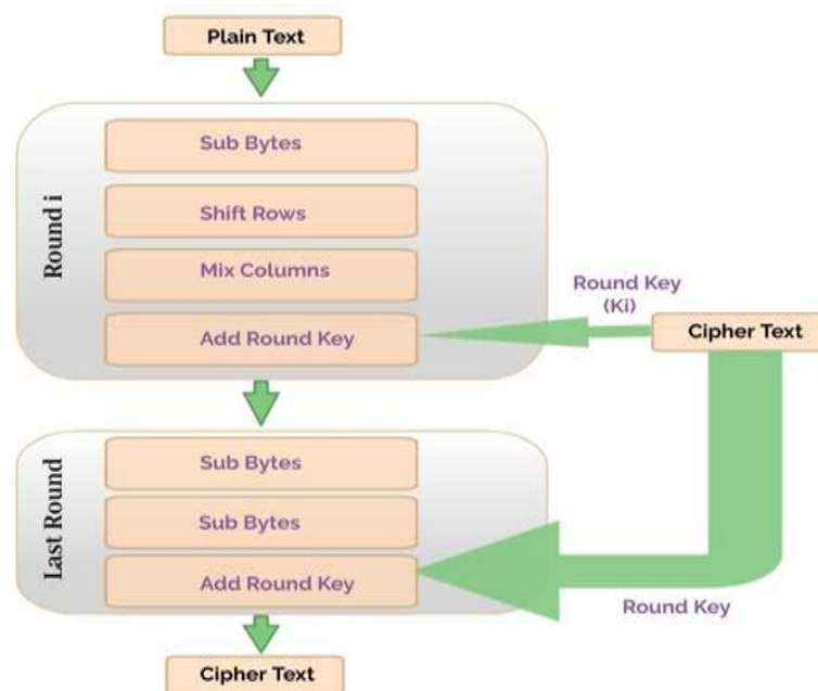
Figure.1. AES Algorithm and its Diagrammatic Representation
